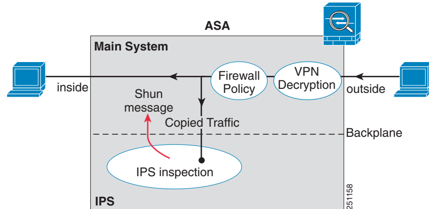
Figure 55-2 IPS Module Traffic Flow in the Adaptive Security Appliance: Promiscuous Mode
