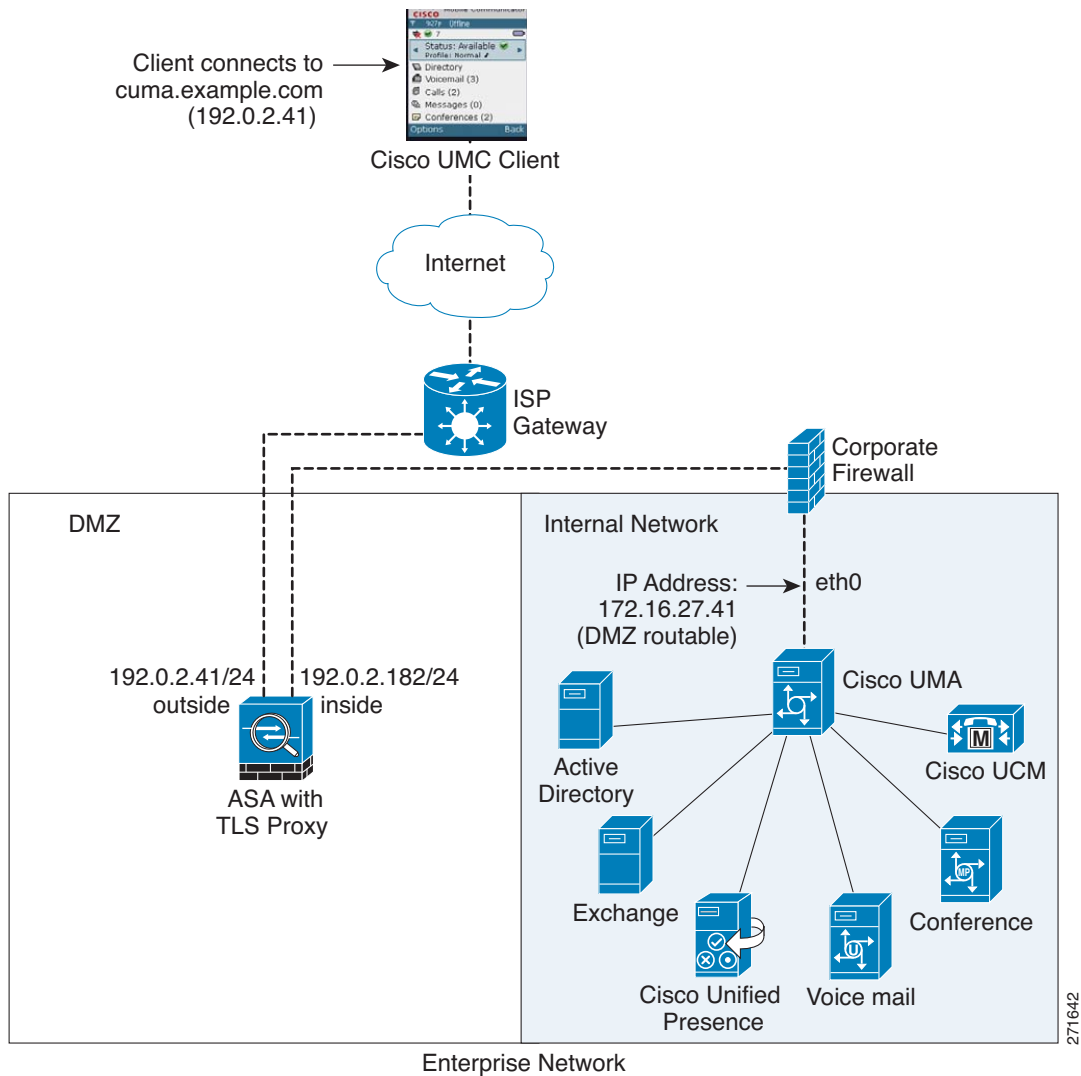
Figure 46-7 Cisco UMC/Cisco UMA Architecture – Scenario 2: Security Appliance as TLS Proxy Only
