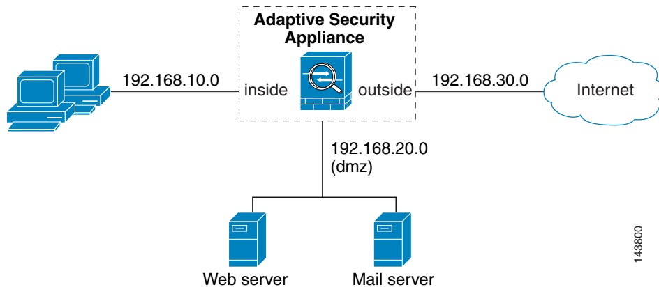
Figure 56-3 Common Network Configuration for CSC SSM Scanning
