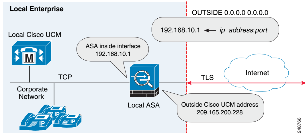
Figure 48-9 Example for Configuring Off Path Signaling in an Off Path Deployment
