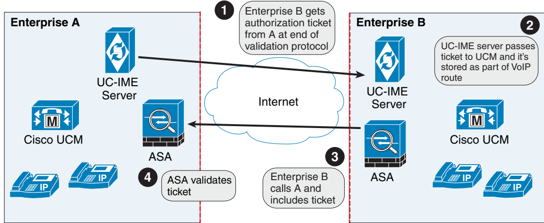
Figure 48-2 Ticket Verification Process with Cisco Intercompany Media Engine
