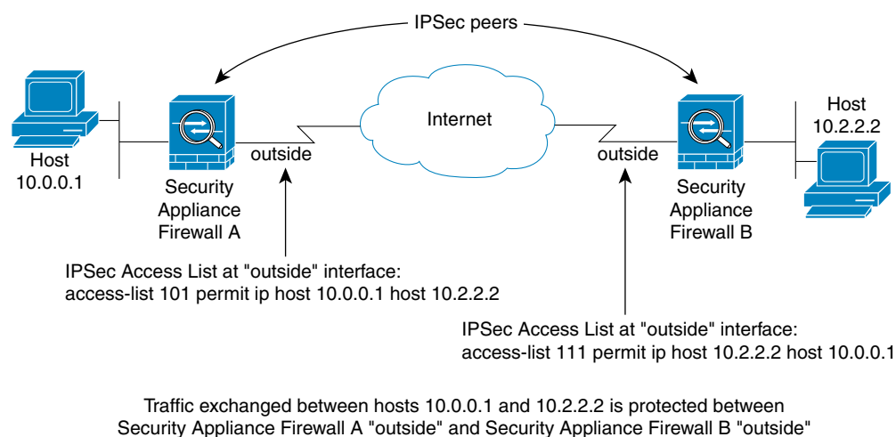
Figure 60-4 How Crypto Access Lists Apply to IPsec
