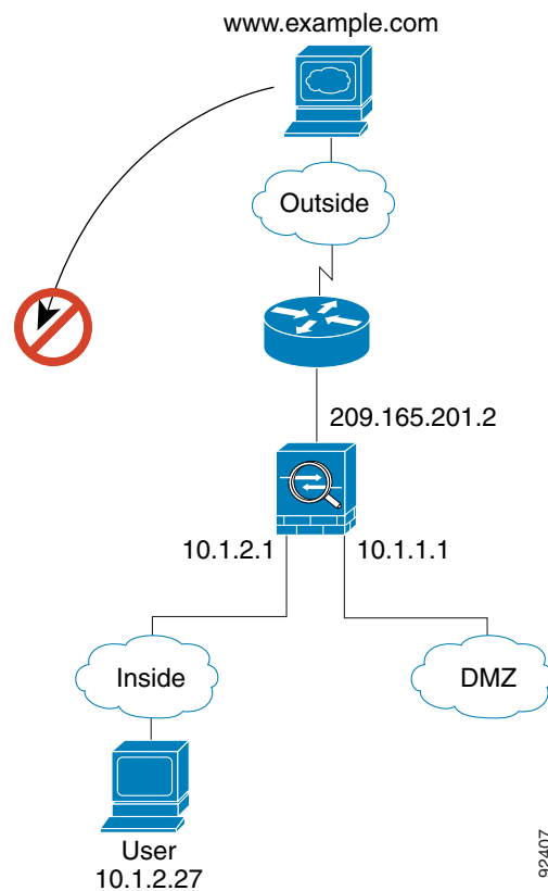
Figure 4-5 Outside to Inside
