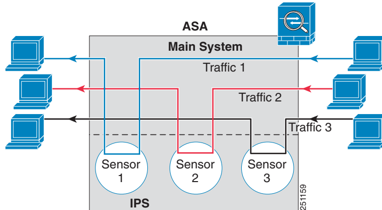
Figure 55-4 Single Mode Security Appliance with Multiple Virtual Sensors
