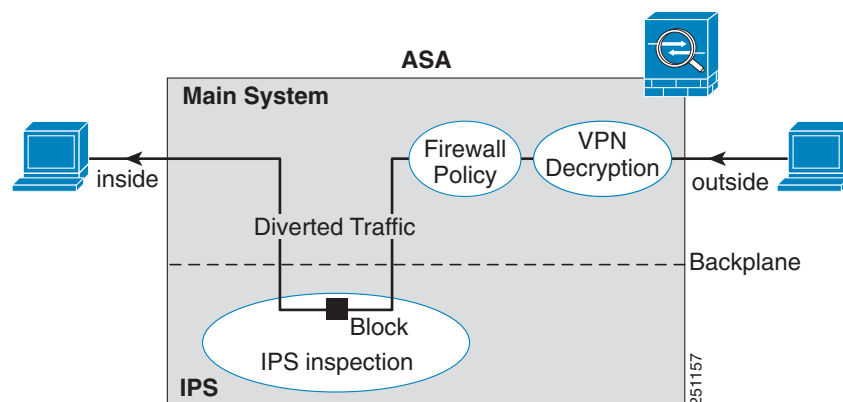
Figure 55-1 IPS Module Traffic Flow in the Adaptive Security Appliance
