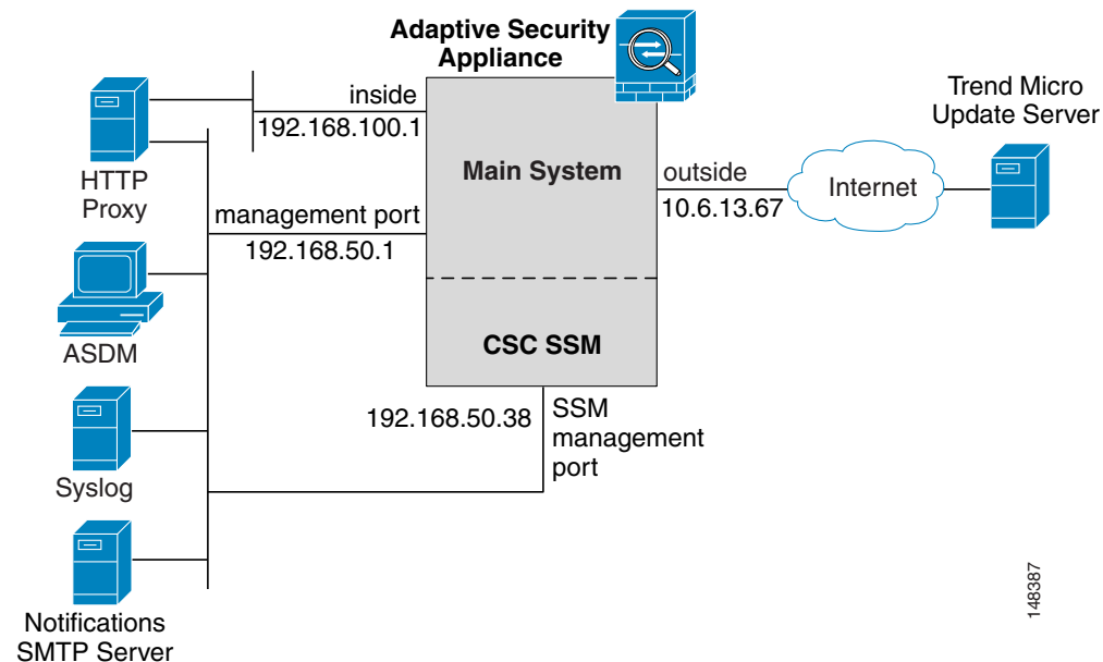
Figure 56-2 CSC SSM Deployment with a Management Network
