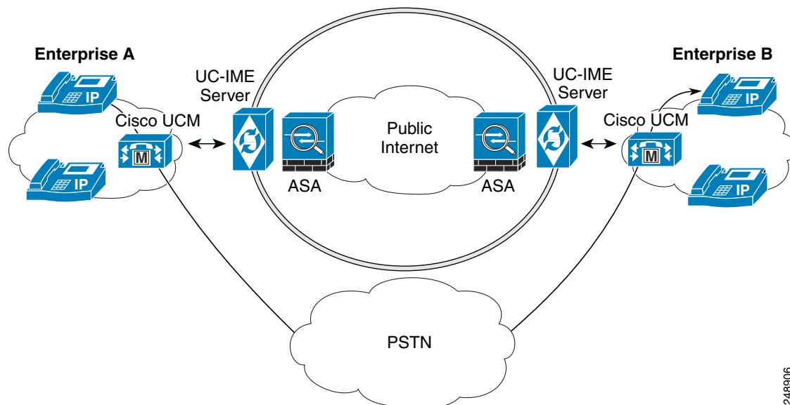
Figure 48-1 Interaction of the UC-IME Proxy with the PSTN
