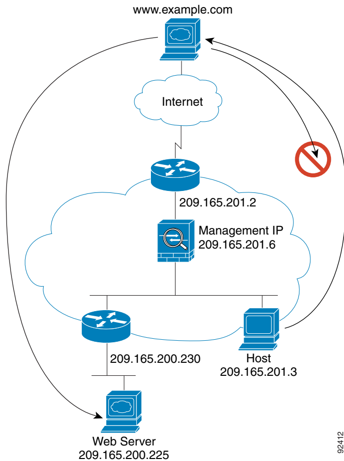
Figure 4-7 Typical Transparent Firewall Data Path
