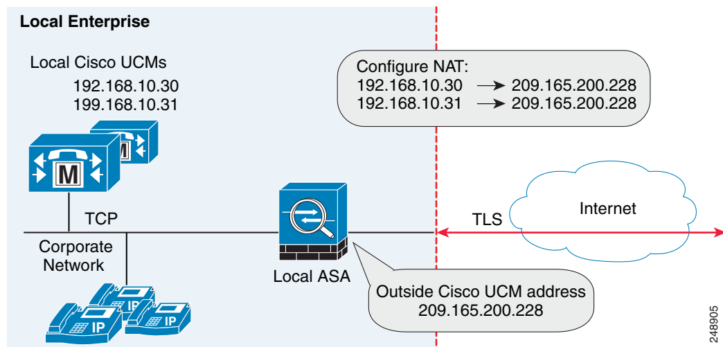
Figure 48-7 Example for Configuring NAT for a Deployment
