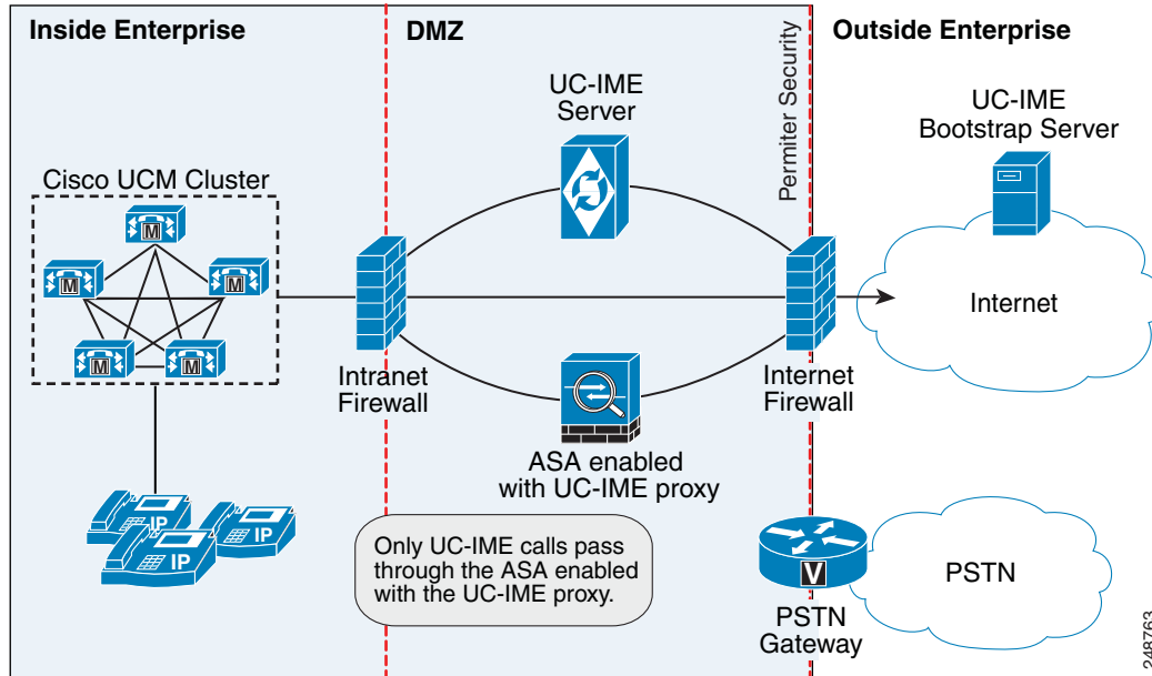
Figure 48-5 Off Path Deployment of the Adaptive Security Appliance
