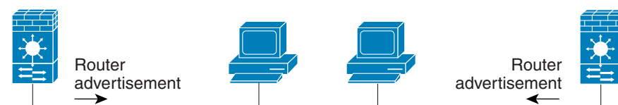
Figure 26-2 IPv6 Neighbor Discovery—Router Advertisement Message
