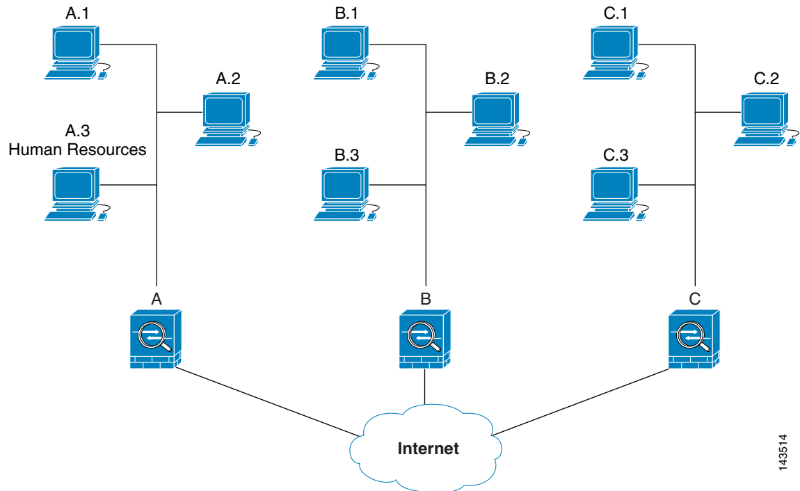
Figure 60-1 Effect of Permit and Deny ACEs on Traffic (Conceptual Addresses)
