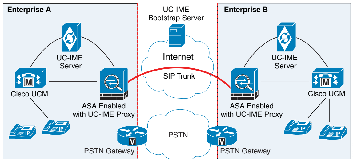
Figure 48-4 Basic Deployment Scenario
