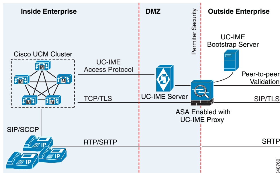
Figure 48-3 Cisco Intercompany Media Engine Architecture in a Basic Deployment
