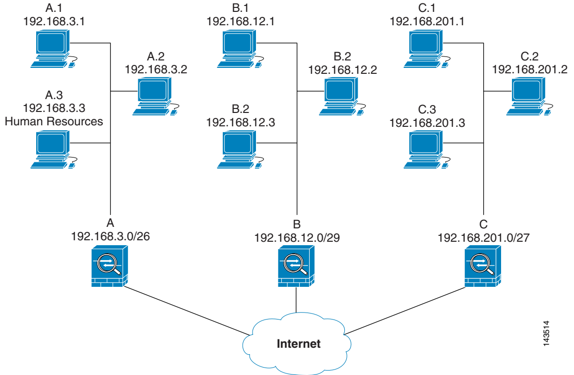
Figure 60-3 Effect of Permit and Deny ACEs on Traffic (Real Addresses)
