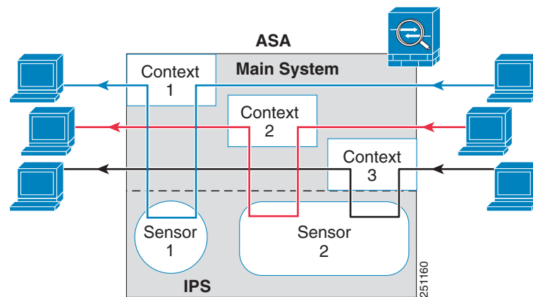
Figure 55-3 Security Contexts and Virtual Sensors
