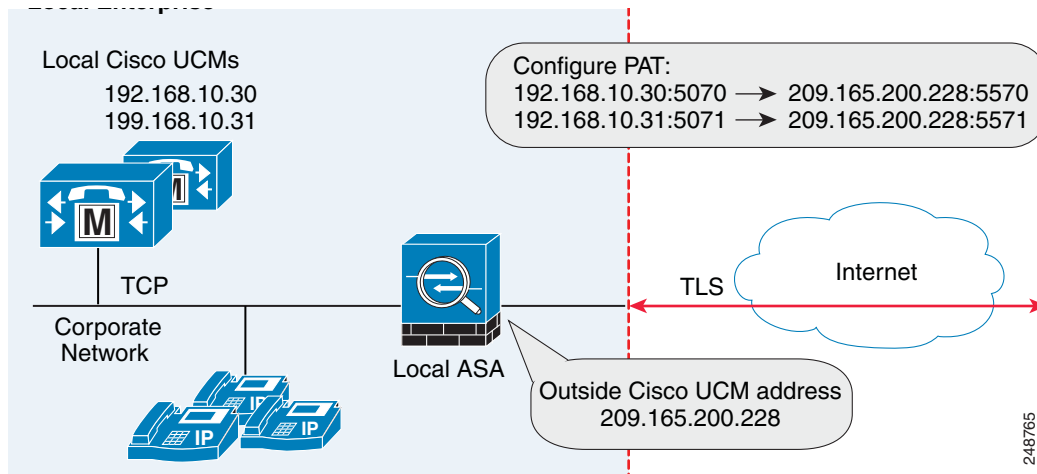
Figure 48-8 Example for Configuring PAT for a Deployment
