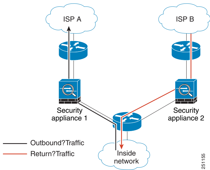
Figure 49-1 Asymmetric Routing
